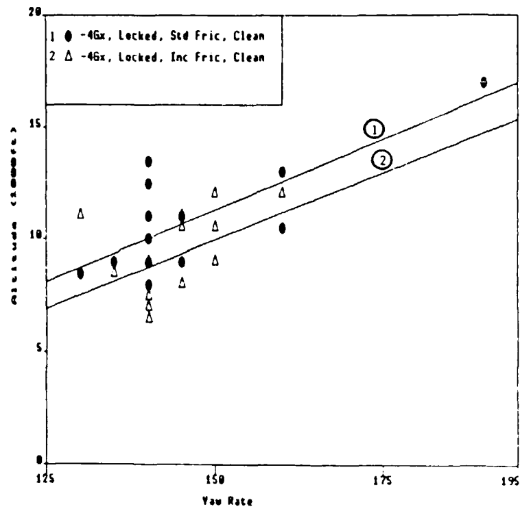
Figure 12: Throttle Friction: Altitude Losses
